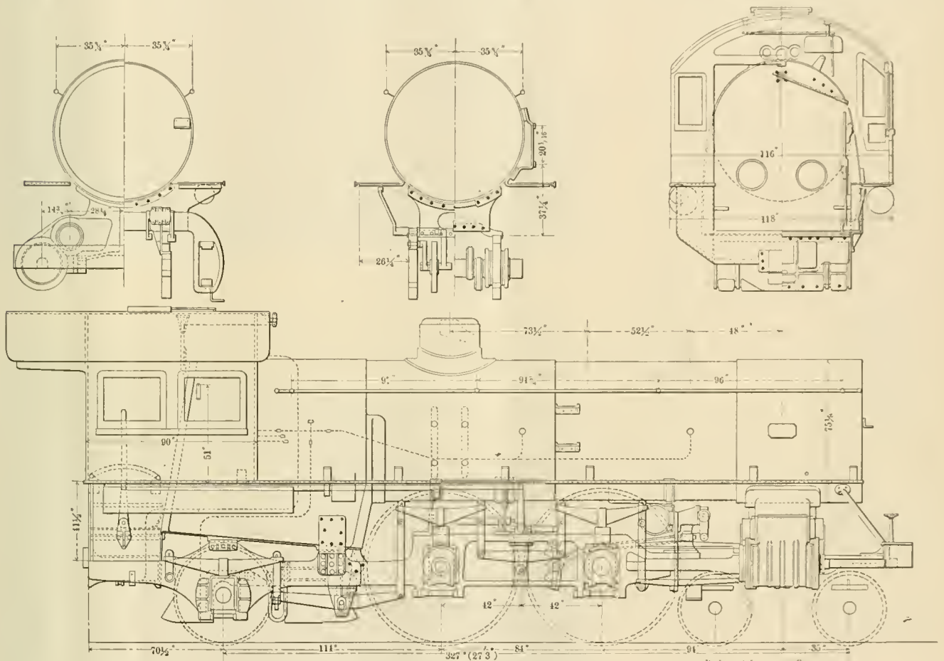
DETAILS OF NEW YORK CENTRAL ENGINE No. 2950. (ILLUSTRATED IN THE JANUARY INSERT.)
